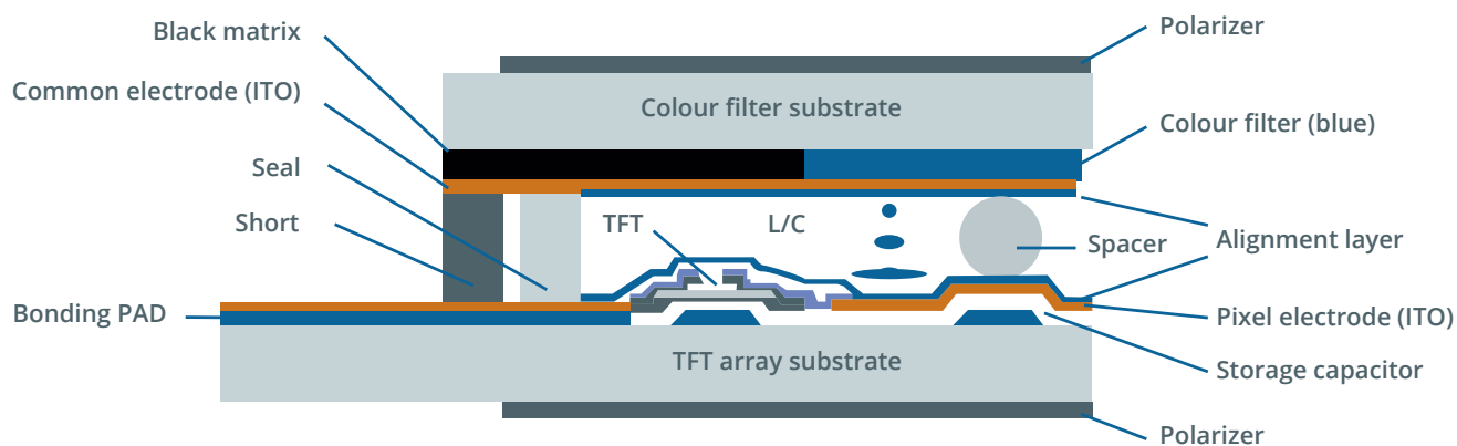
LCD structure
